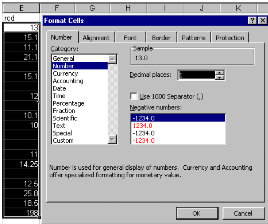
Figure 11 - Formatting data
